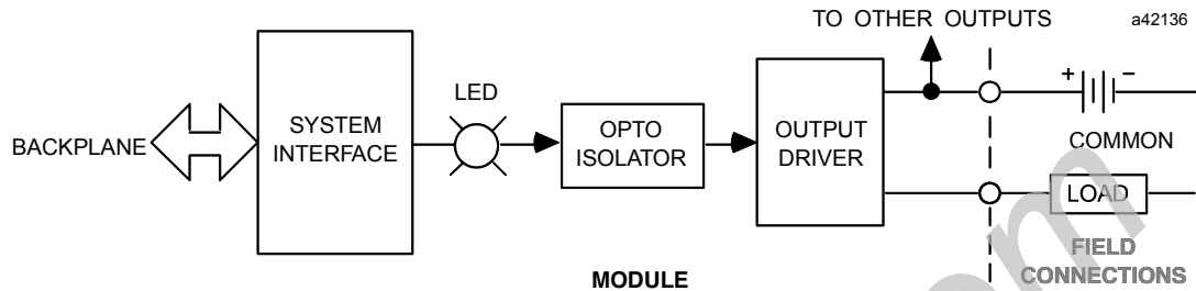
Figure 1. Block Diagram for IC697MDL750
