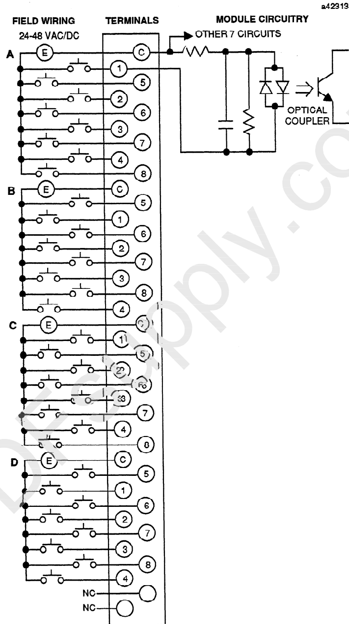
Figure 16. Field Wiring and Typical Circuit for IC655MDL512
