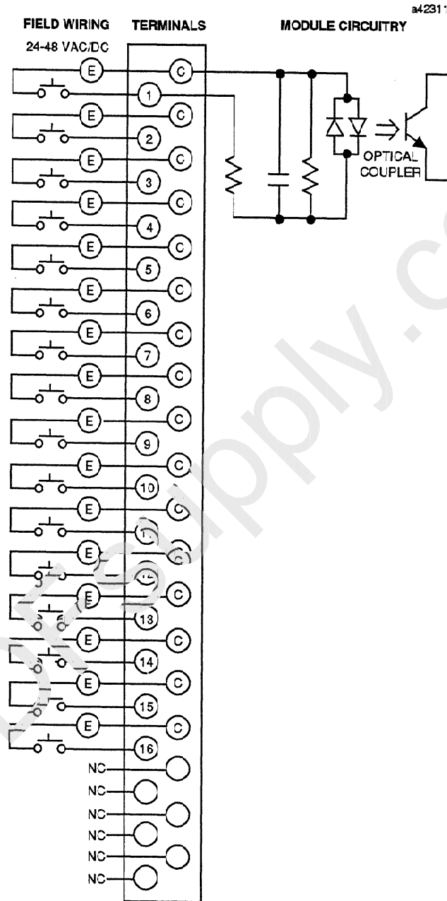
Figure 14. Field Wiring and Typical Circuit for IC655MDL511
