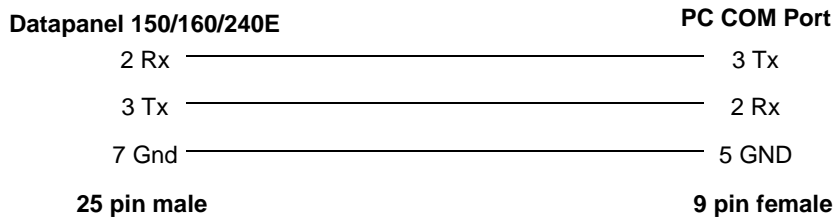
Figure 2-2. Download Cable
