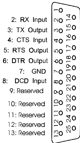
25 pin Serial Port Model 240T
