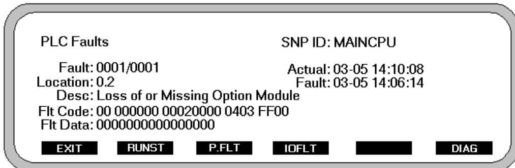
Figure 6-4. PLC Faults Log– Model 320T
