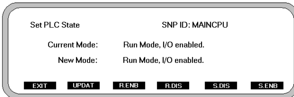
Figure 6-6. PLC Run/Stop Mode Screen – Model 320T
