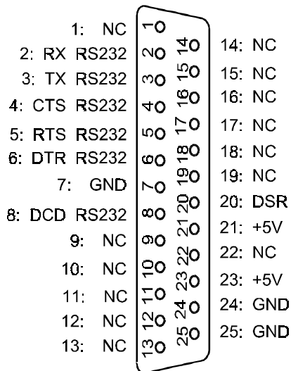
Figure 7-2. Model 320T Base Ports and Pinouts
