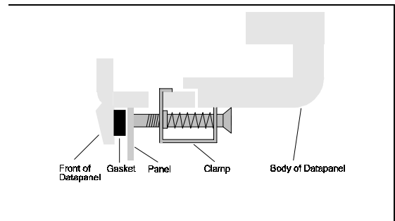
Clamp Mounting Detail
