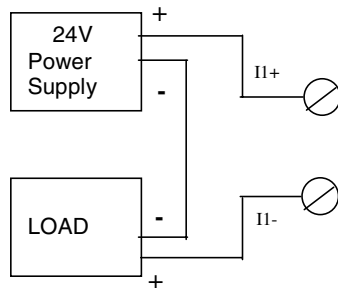
Current Source
