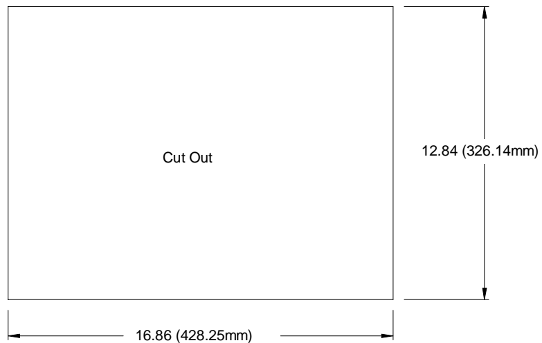
Figure 2. Panel Cutout Dimensions
