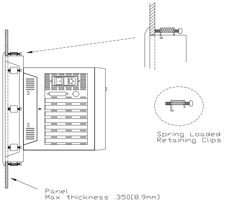
Figure 3. Mounting the Touch Display Unit
