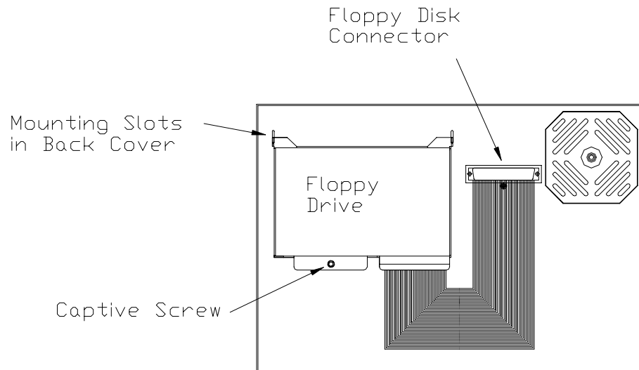
Figure 5. Floppy Disk Drive Mounting
