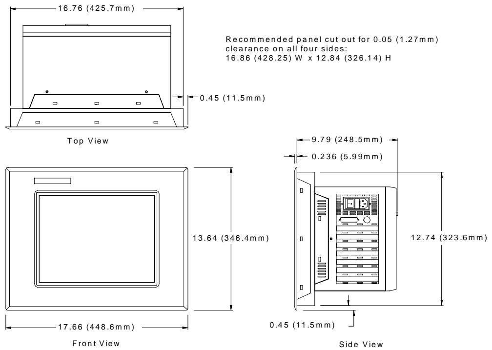
Figure 1. Touch Display Unit Dimensions
