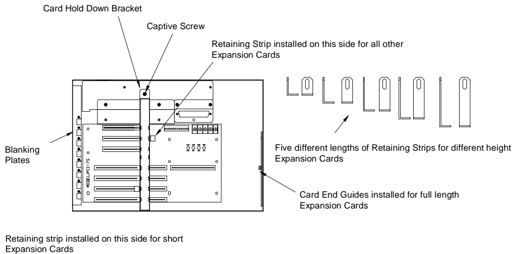
Figure 4. Card Clamp Chassis
