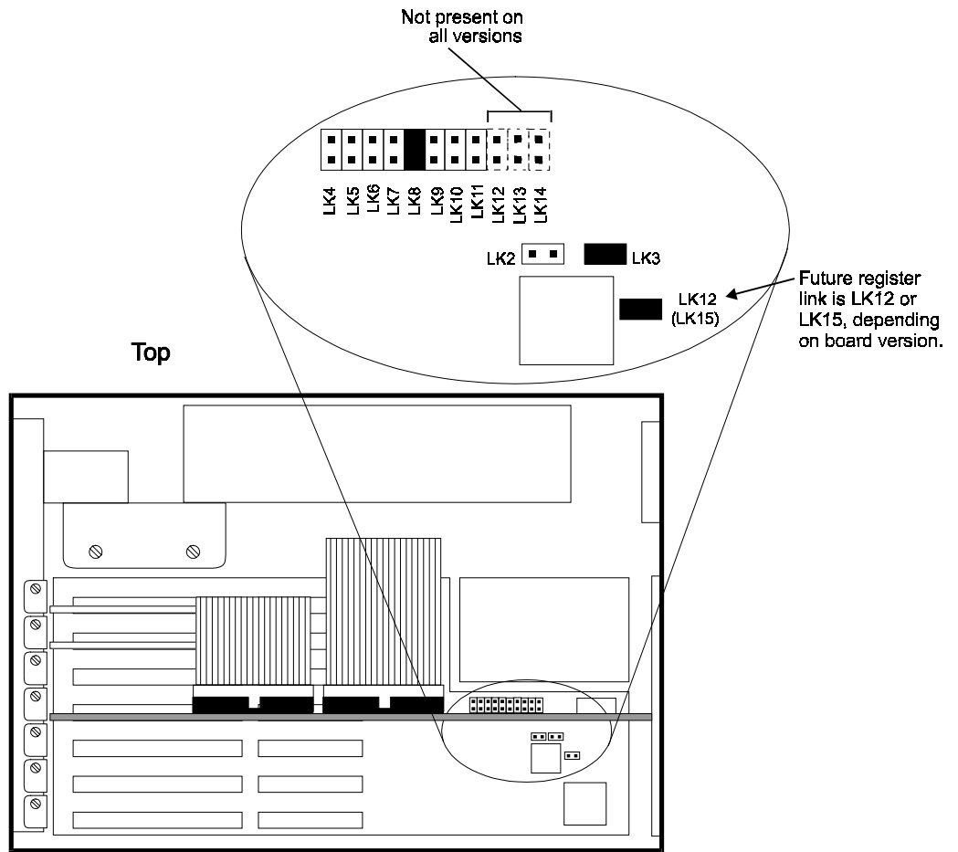
Figure 5. Jumper Locations
