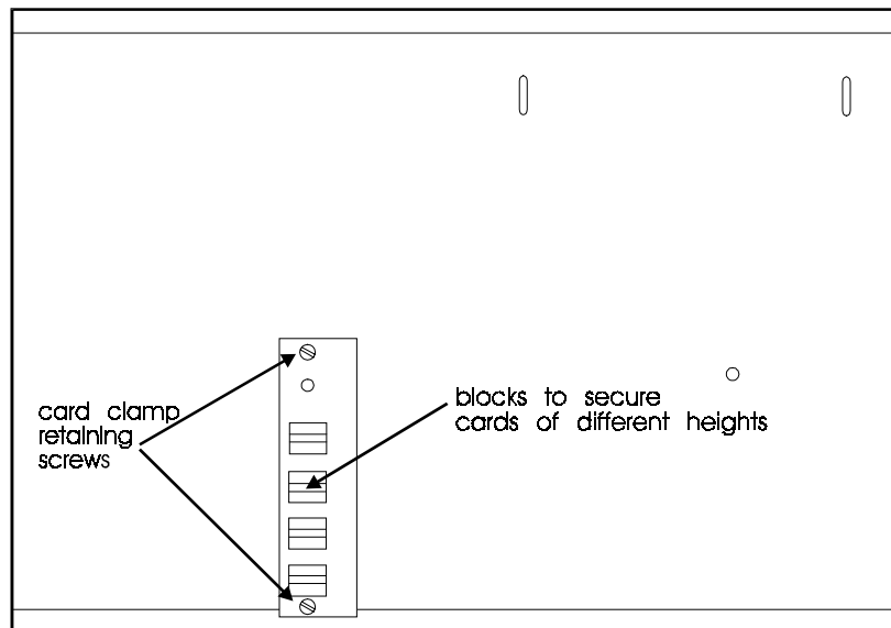
Figure 4. Card Clamp
