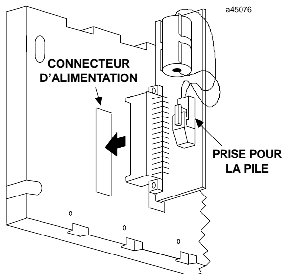
Figure 1-26. Installation du kit de pile
