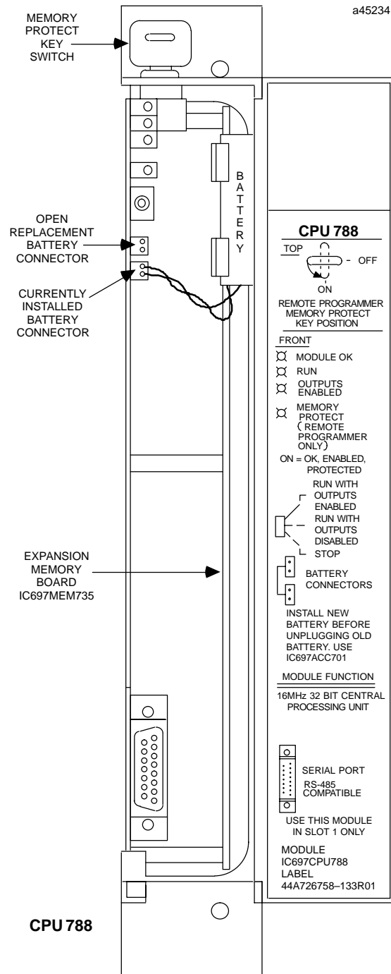
Figure 2. CPU 788 - Location of Major Features
