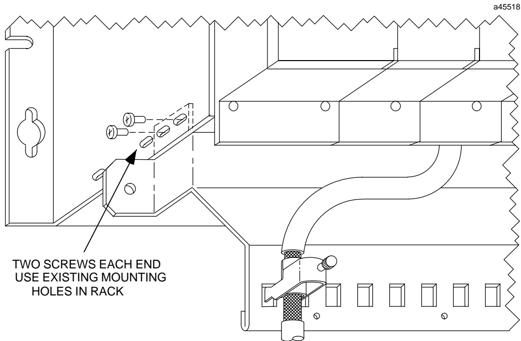
Figure 5. Cable Shield Clamping Assembly Mounted on an IC697 Rack
