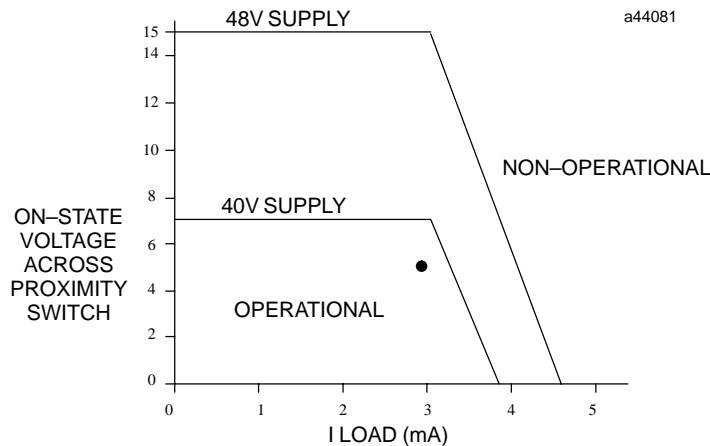
Figure 2. Proximity Switch Compatibility
