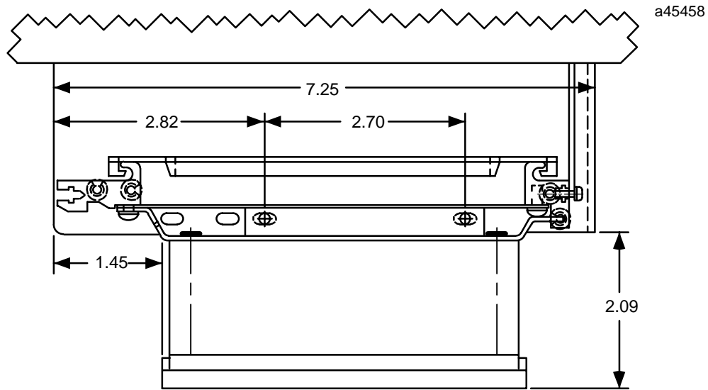
Figure 3. Fan Assembly Dimensions for Mounting
