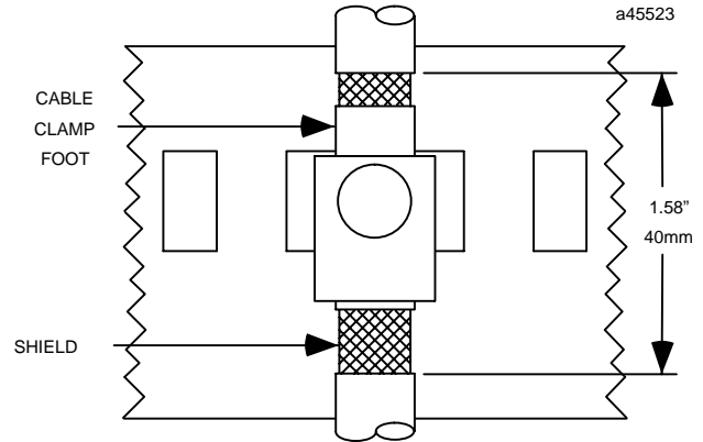
Figure 4. Clamped Cable with Exposed Shield
