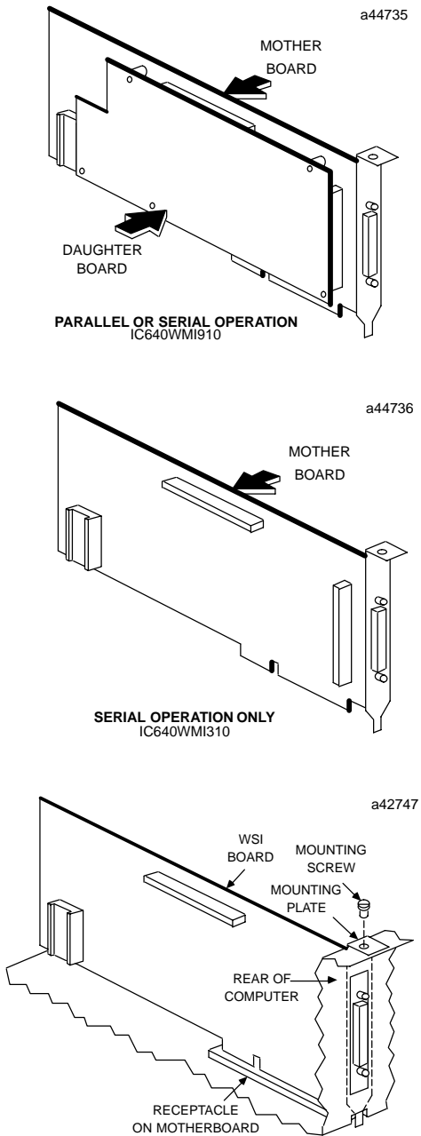
Figure 2. WSI Installation in IC640 Computer
