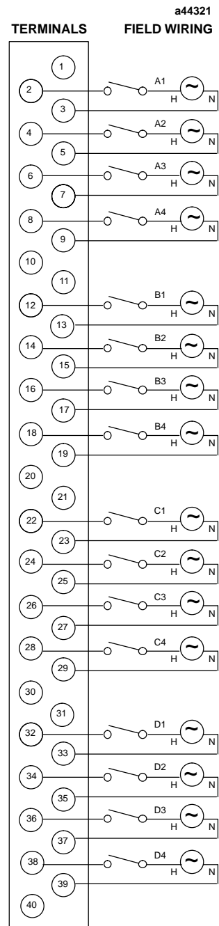
Figure 3. Field Wiring Connections for IC697MDL241
