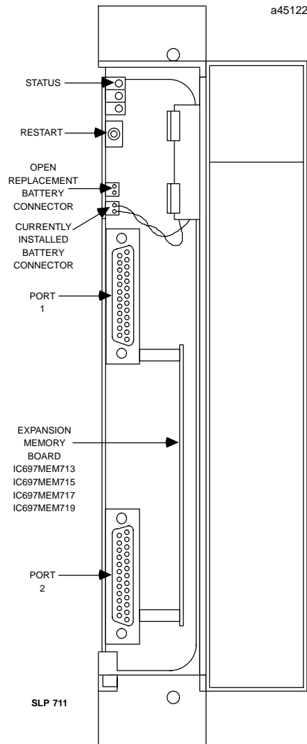
Figure 2. State Logic Processor Module, User Details Programming and Configuration
