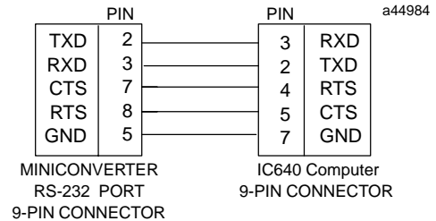
Figure 3. Miniconverter to 9-Pin IC640 Computer or PC-XT Computer (Additional Adapter Required)
