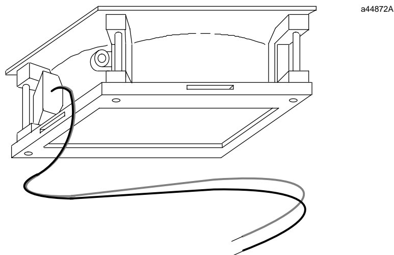
Figure 6. Wire Lead Detail for Fans in the IC697ACC744 24 VDC Rack Fan Assembly
