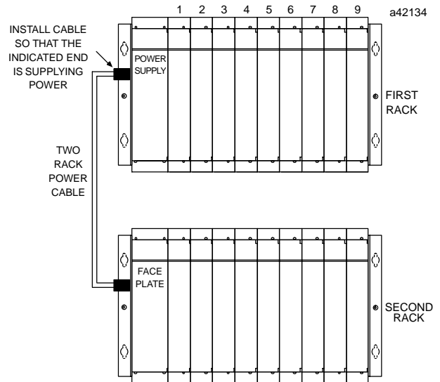
Figure 2. Dual Rack Configuration
