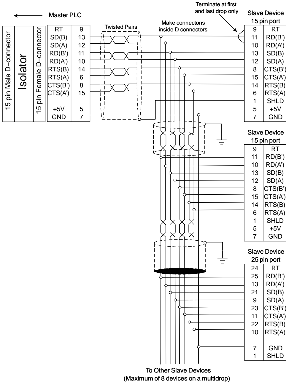
Figure 5. Multidrop Configuration Connecting Devices with 15-Pin Ports and 25-Pin Ports
