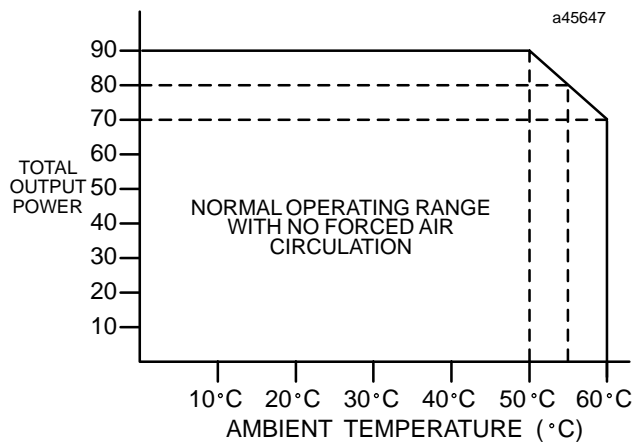
Figure 7. Output Power Derating Curve
