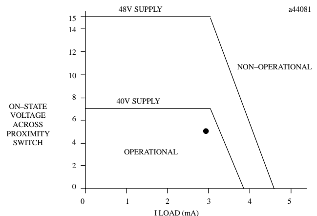
Figure 2. Proximity Switch Compatibility
