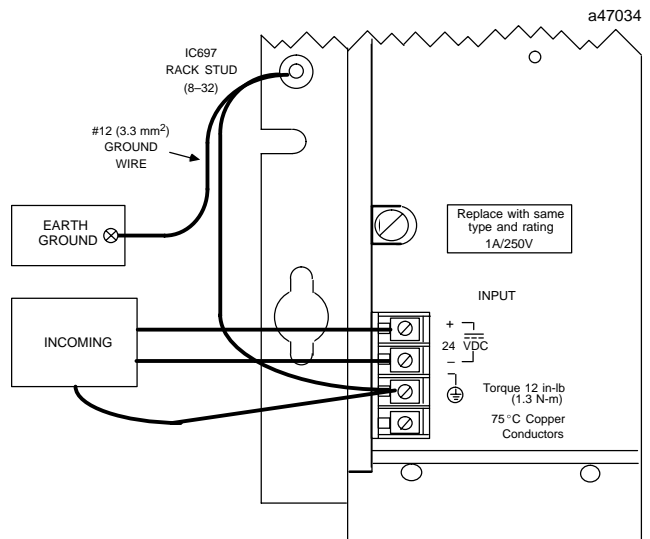
Figure 10. Input Wiring and Ground Connections
