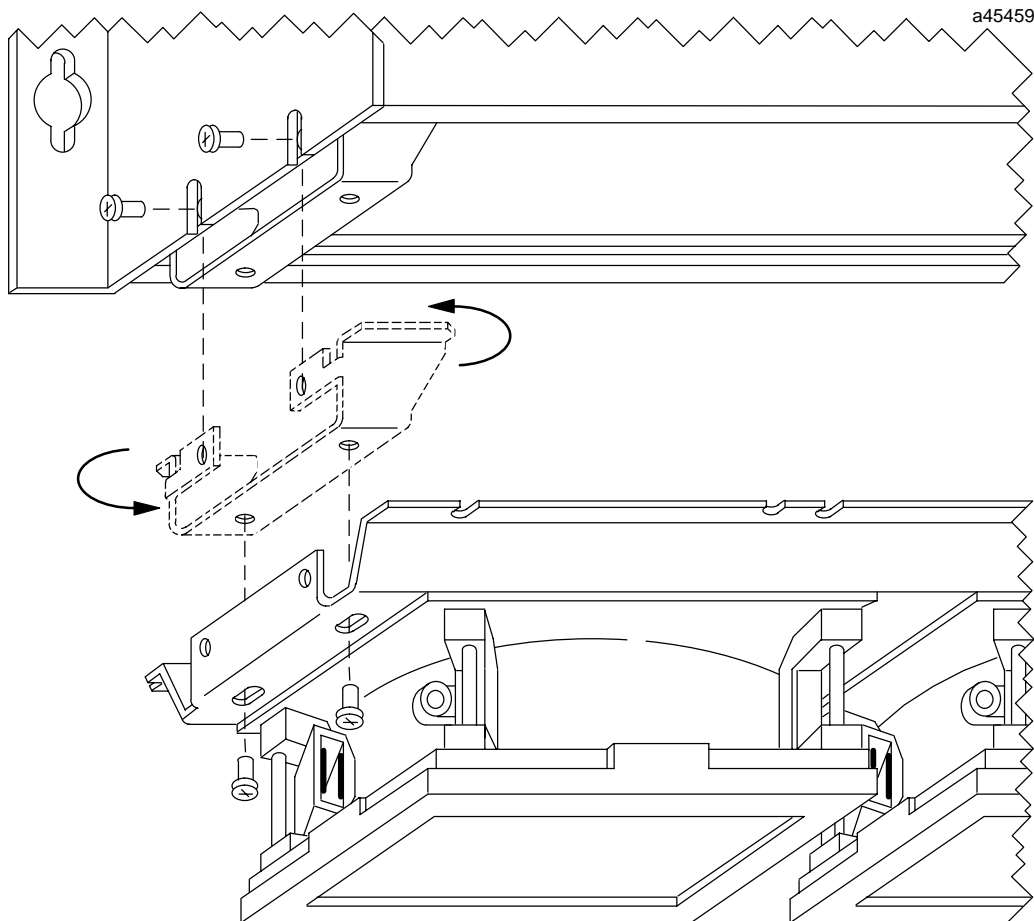
Figure 4. Mounting Details for Fan Assembly (AC Type Shown) and Optional Mounting Bracket
