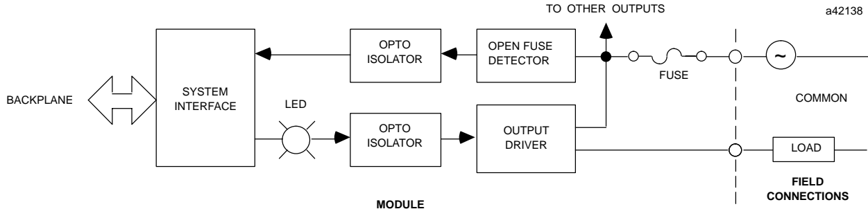
Figure 1. Block Diagram for IC697MDL350
