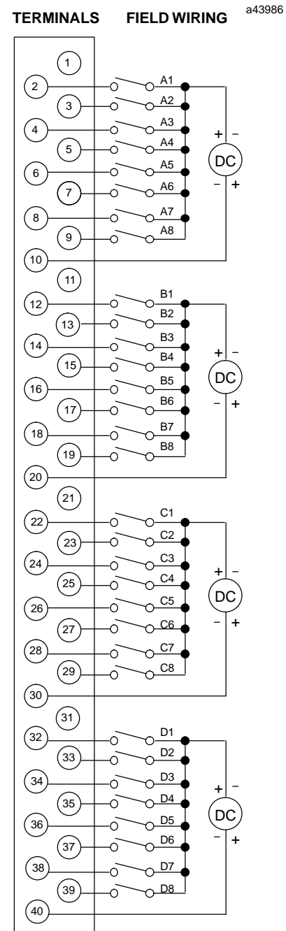
Figure 3. Field Wiring Connections
