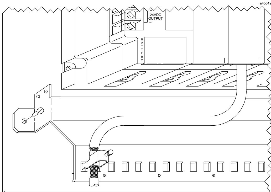
Figure 2. Example of Cable Shield Clamping Assembly Installation
