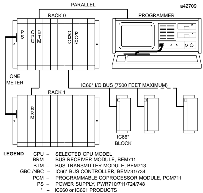
Figure 3. Typical IC697 PLC System Configuration
