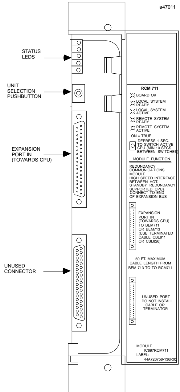
Figure 2. Redundancy Communications Module User Details
