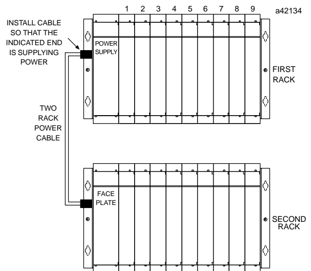
Figure 8. Dual Rack Configuration
