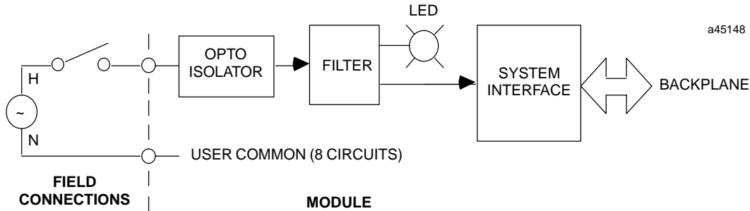
Figure 1. Block Diagram for IC697MDL254
