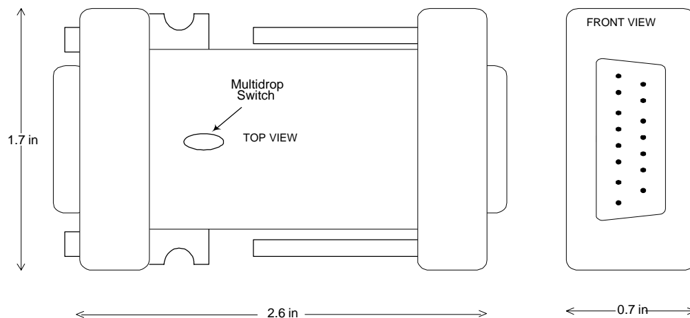
Figure 1. RS-485 Port Isolator
