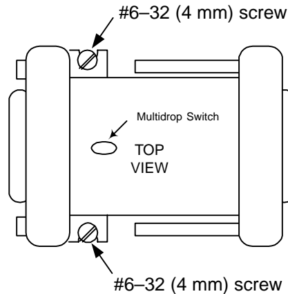
Figure 4. Mounting Port Isolator to Panel
