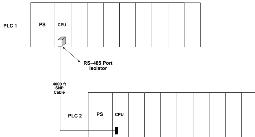
Figure 3. RS-485 Port Isolator in PLC Network
