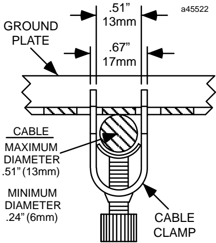
Figure 3. Cross Section of Cable Secured by Clamp
