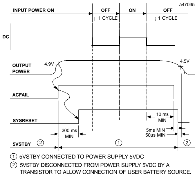
Figure 9. Timing Diagram for 24 VDC Power Supply
