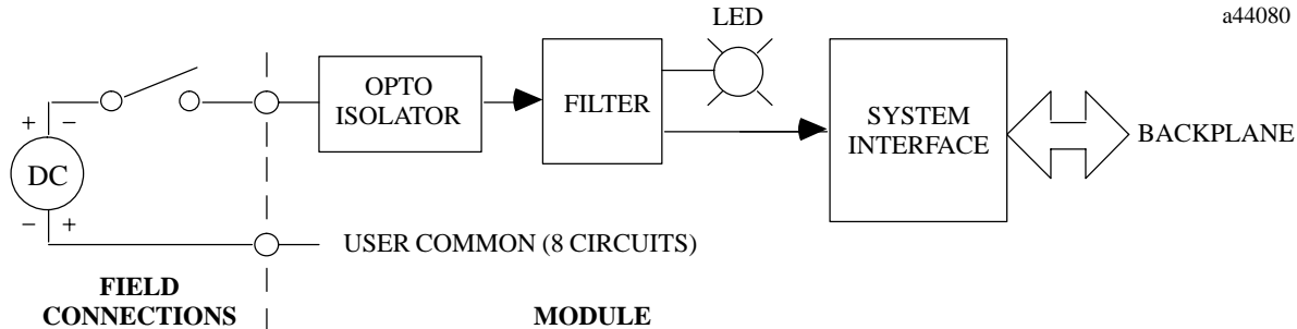
Figure 1. Block Diagram for IC697MDL654
