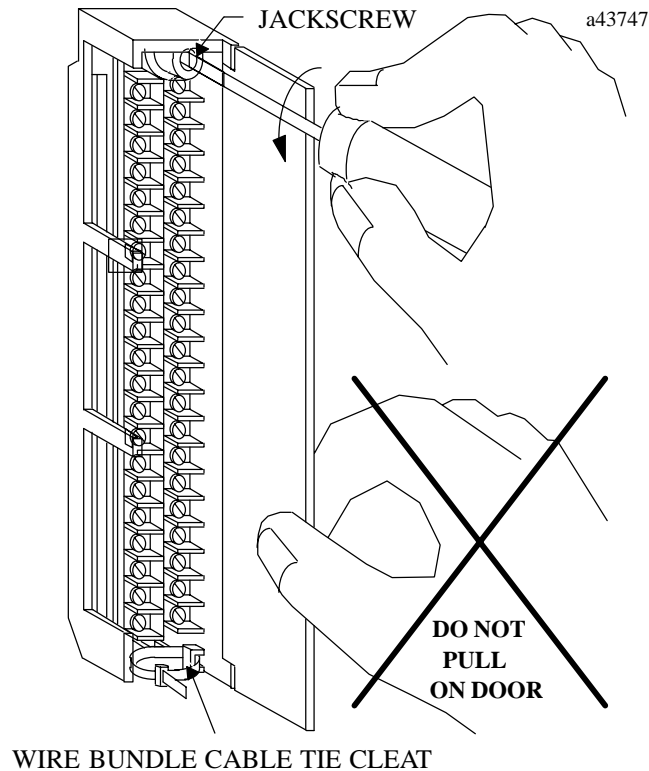
Figure 5. Removal of I/O Terminal Board
