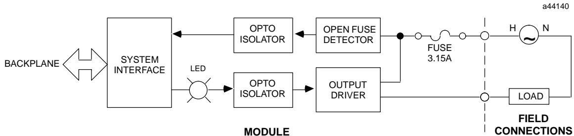
Figure 1. Block Diagram for IC697MDL341
