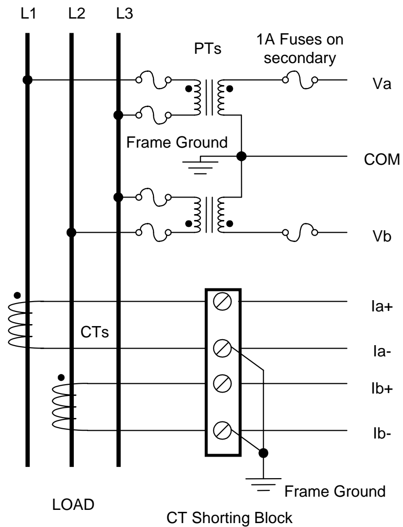
Figure 3-7. Configuration for 3-Phase 3-Wire Delta system with 2 PTs
