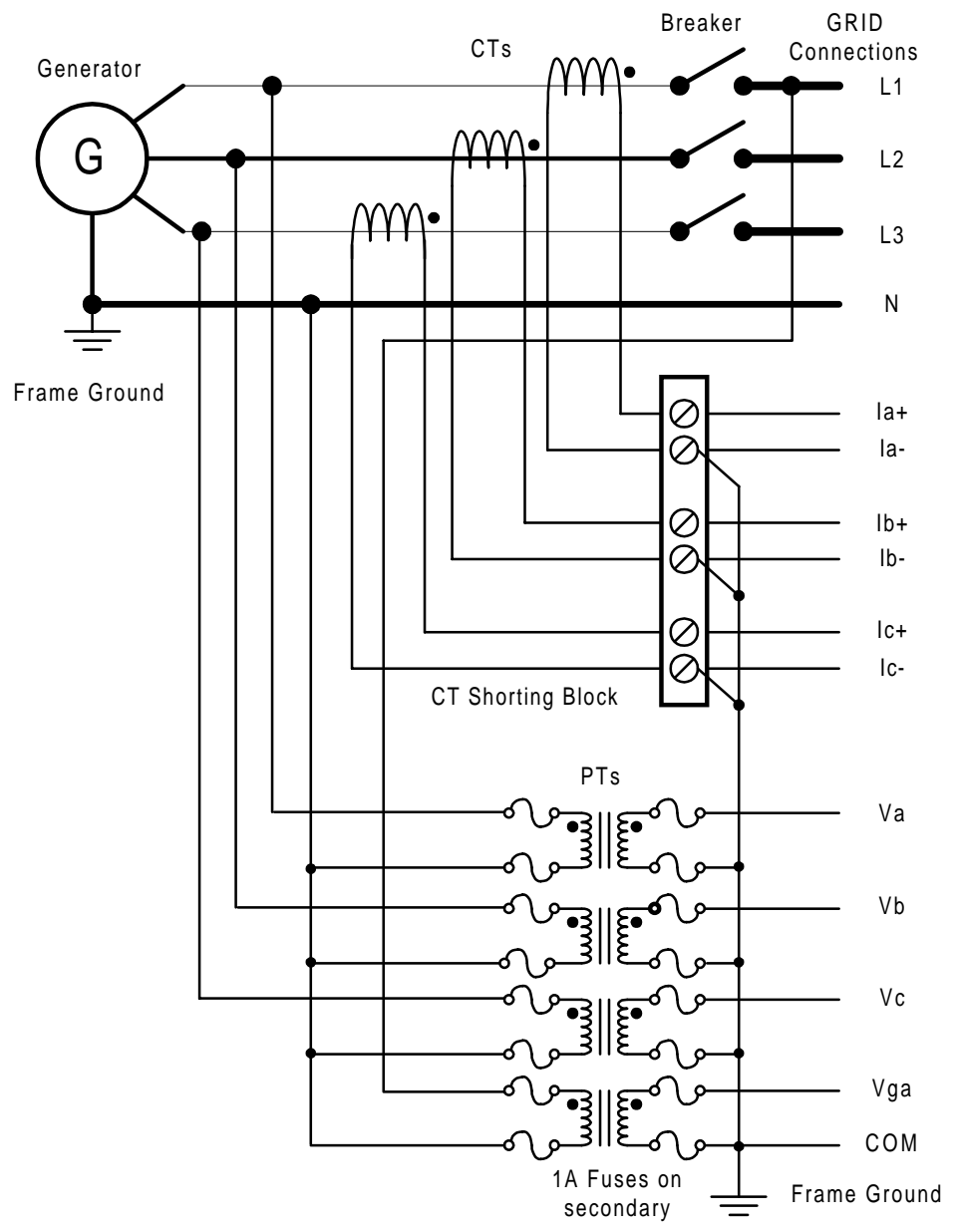
Figure 3-8. Wye Synchro/Power Monitor connection
