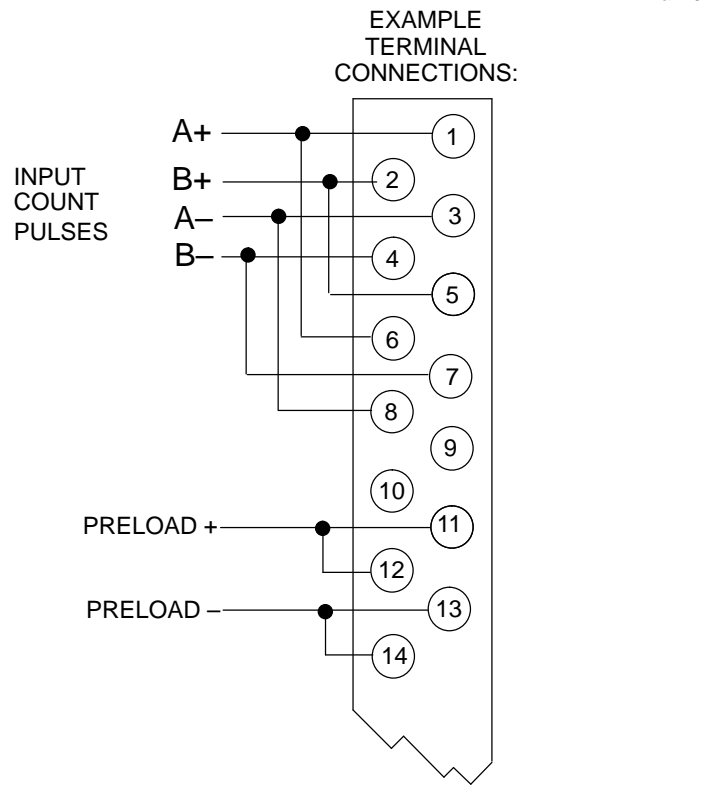
Figure E-3. Example of Terminal Connections
