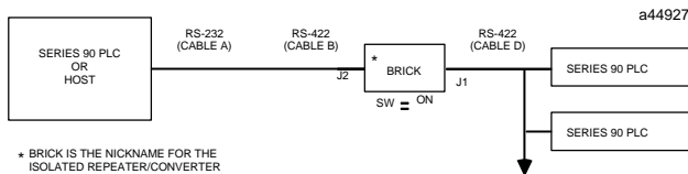
Figure A-8. Simple System Configuration Using the Isolated Repeater/Converter
