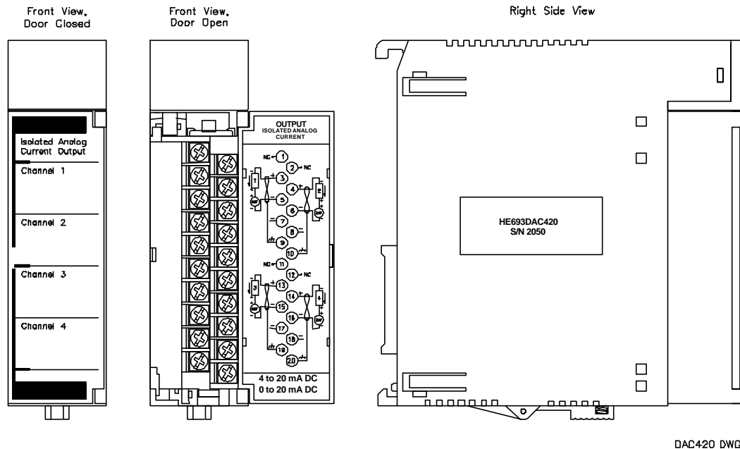
Figure 1 – HE693DAC420 Module
