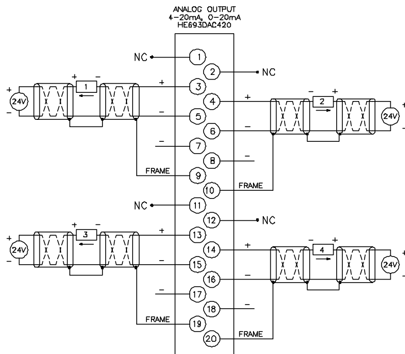
Figure 4 - Wiring
