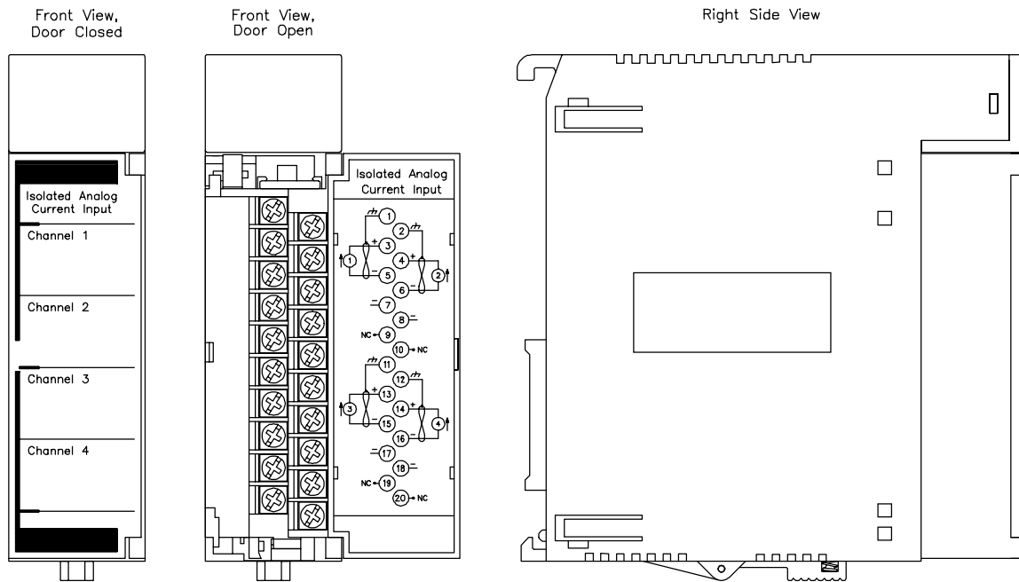
Figure 1 – HE693ADC420 Module
