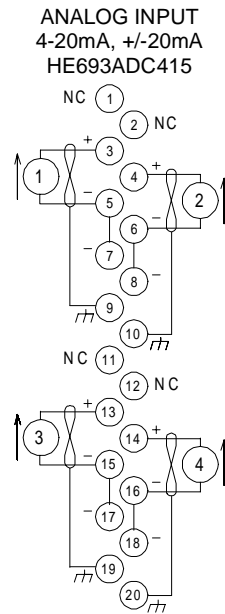
Figure 4 – HE693ADC415 Wiring
