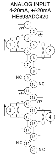
Figure 5 – HE693ADC420 Wiring
